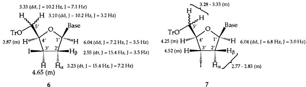
Figure 1. ^1\text{H} NMR of 6 and 7 in \text{DMSO-d}_6 , expressed in \delta (ppm) downfield from tetramethylsilane.
